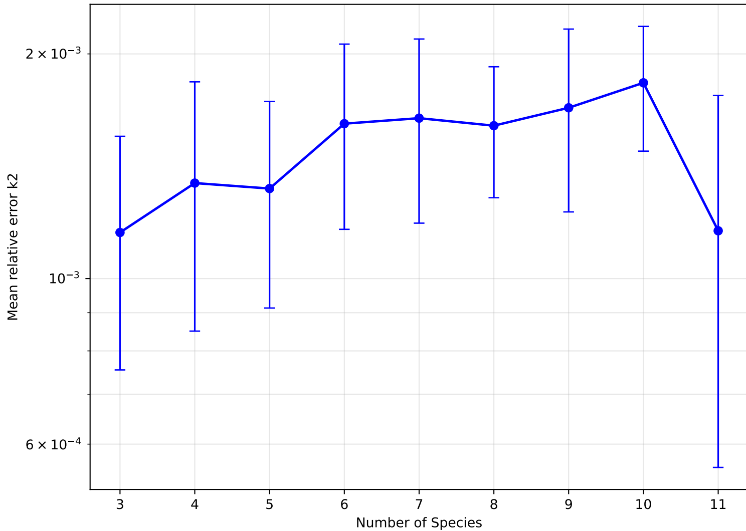
30, 30 — Mean relative error k2 vs number of species (3 to 11 species)
